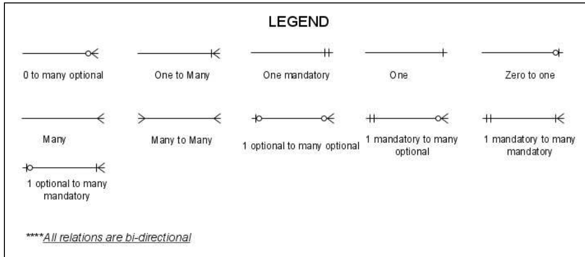
Figure 2: Cardinalities of relationships
