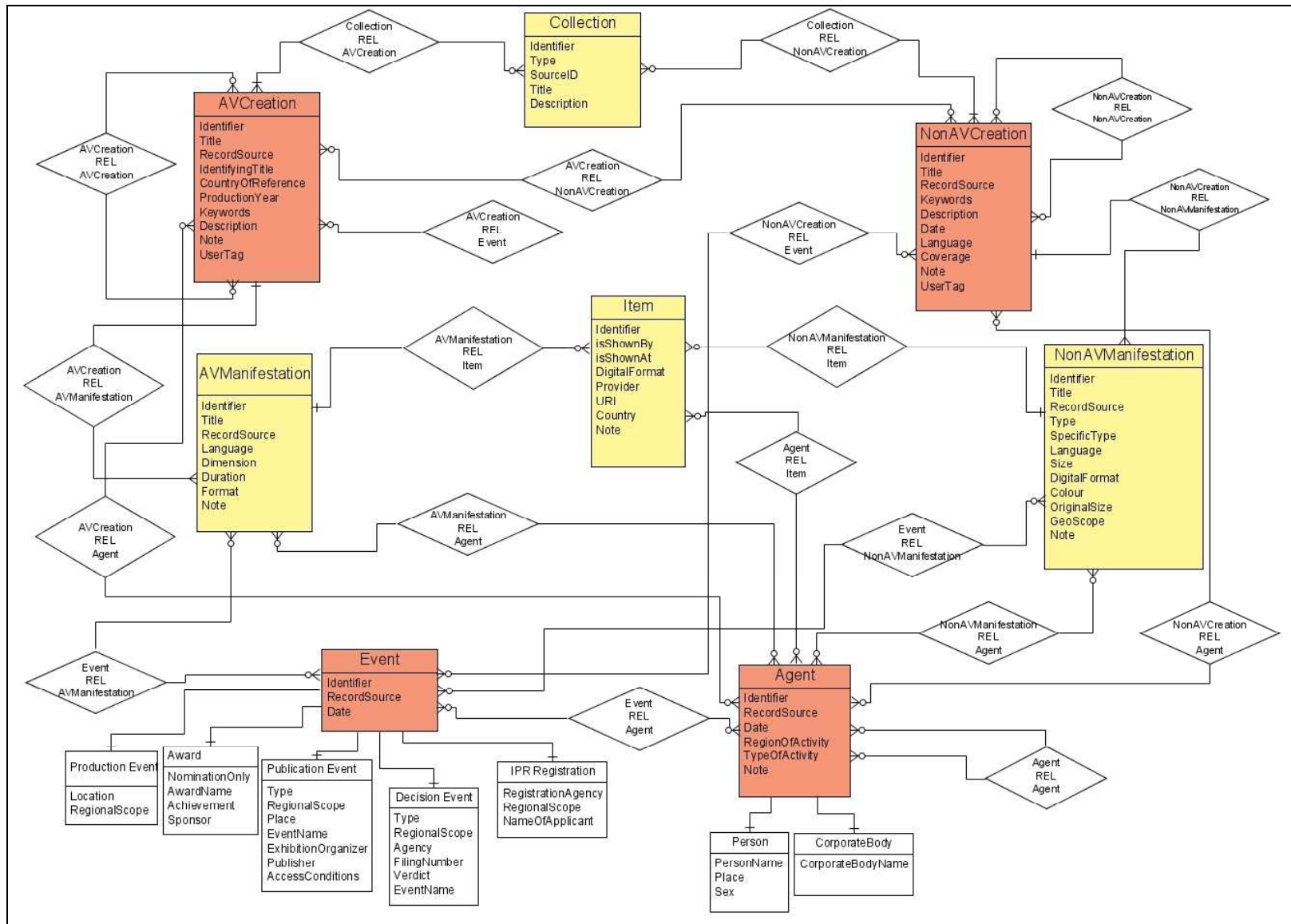
Figure 1: Entities and relationships of the EFG metadata model
