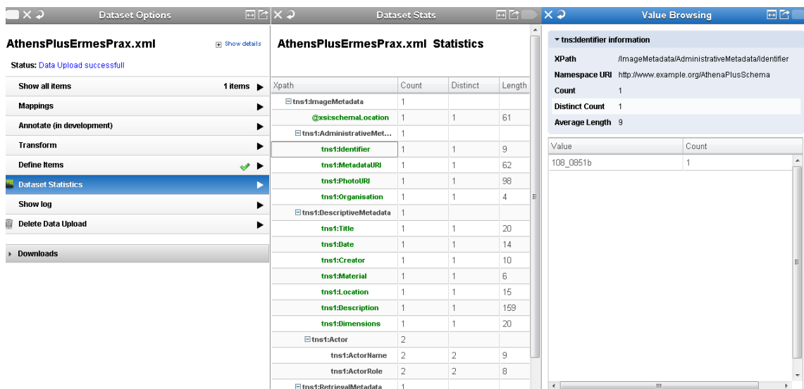
Figure 44: Dataset statistics
