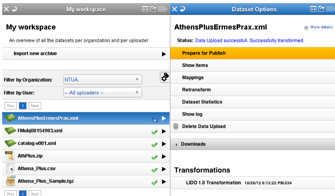
Figure 72: Transformed dataset
