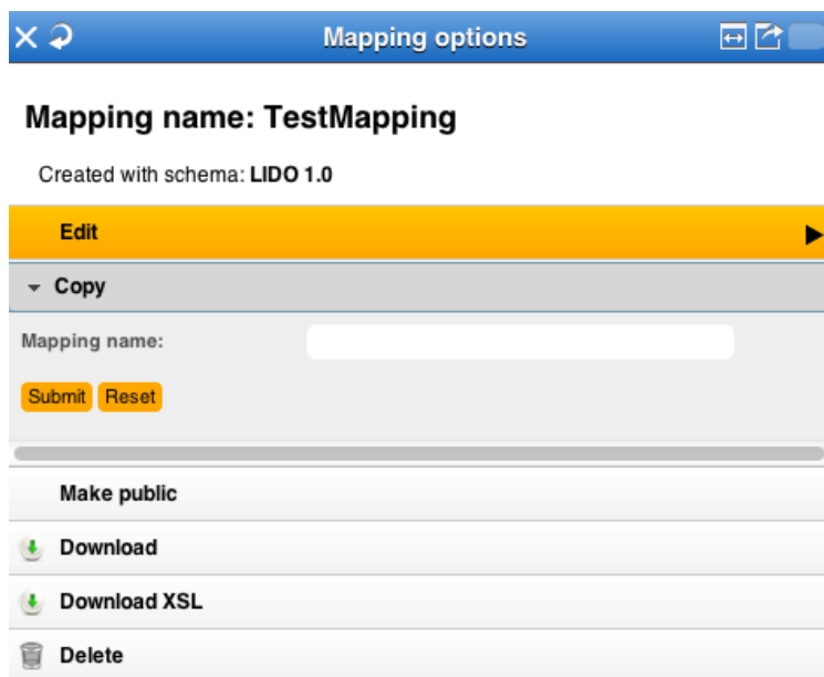
Figure 56: Mappings management
