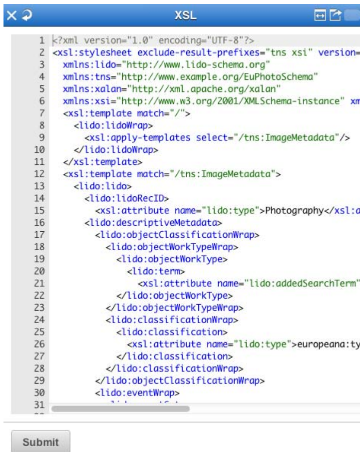
Figure 55: The XSL editor
