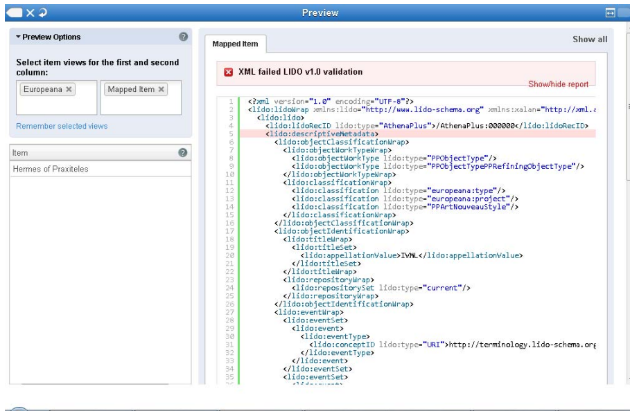
Figure 68: The output preview with an error highlighted
