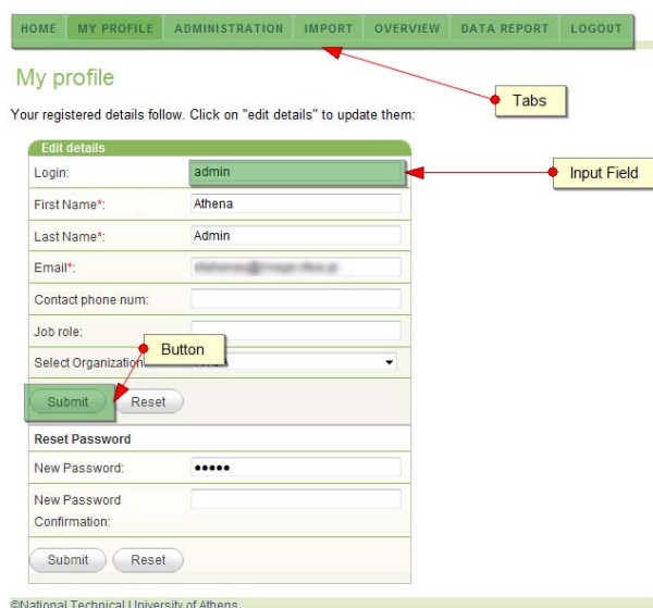
Figure 6: MINT's old user interface
