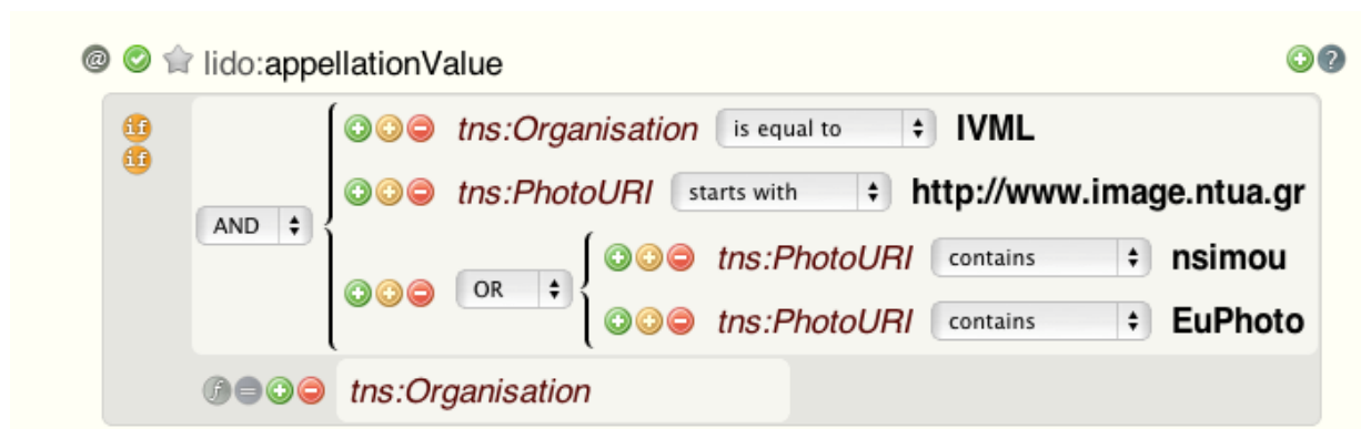
Figure 64: Conditional mapping
