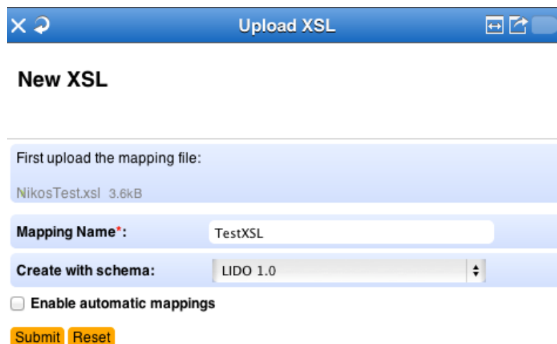
Figure 54: Upload XSL
