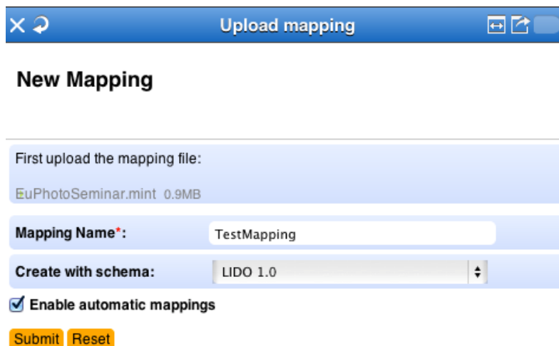
Figure 53: Upload mapping
